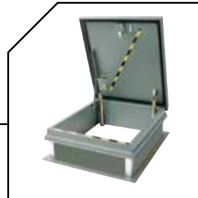
Hatch door opens full on release with one-point locking mechanism
